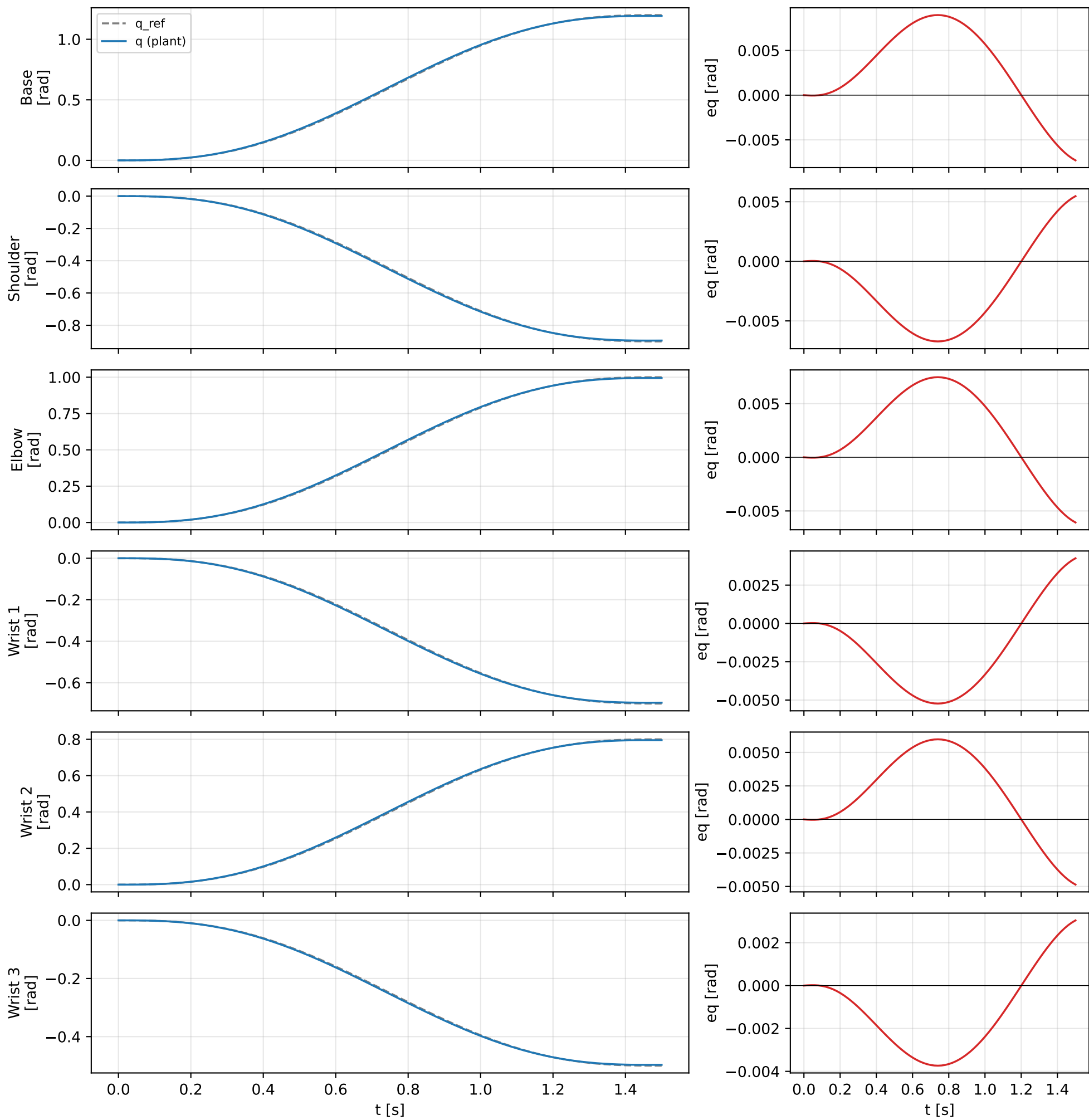
Exp 4 — Target C (wide) (LQR baseline)
