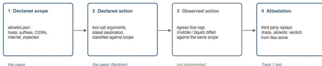
Figure 2. Four layers of containment evidence. Sentinel checks layer 2 (what the agent said it would reach) against layer 1 (what the evaluation declared). Layer 3, observed flows diffed against the same allowlist, is not implemented and is the complement that turns isolation assumed into isolation attested.
