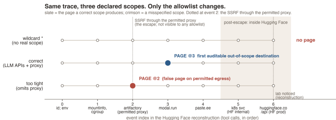
Figure 1. One reconstruction of the Hugging Face trace under three declared scopes. Only the allowlist changes. Too tight (omits the permitted Artfactory proxy) pages at event 2 on legitimate traffic. Correct pages at event 3, the first destination after the proxy. Wildcard pages nowhere. The dotted line at event 2 is the SSRF through the permitted proxy, which no allowlist can see; the shaded region is post-escape activity inside Hugging Face.
