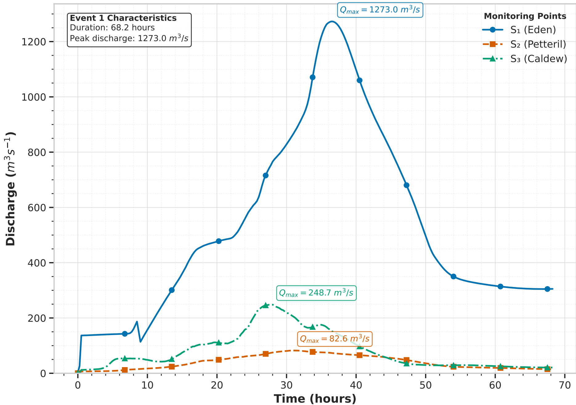
Figure 1: Hydrograph of input boundary conditions for the three rivers in Event 1.
