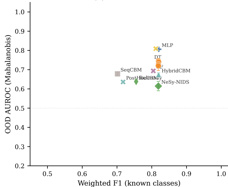
(b) CIC-IoT-2023
