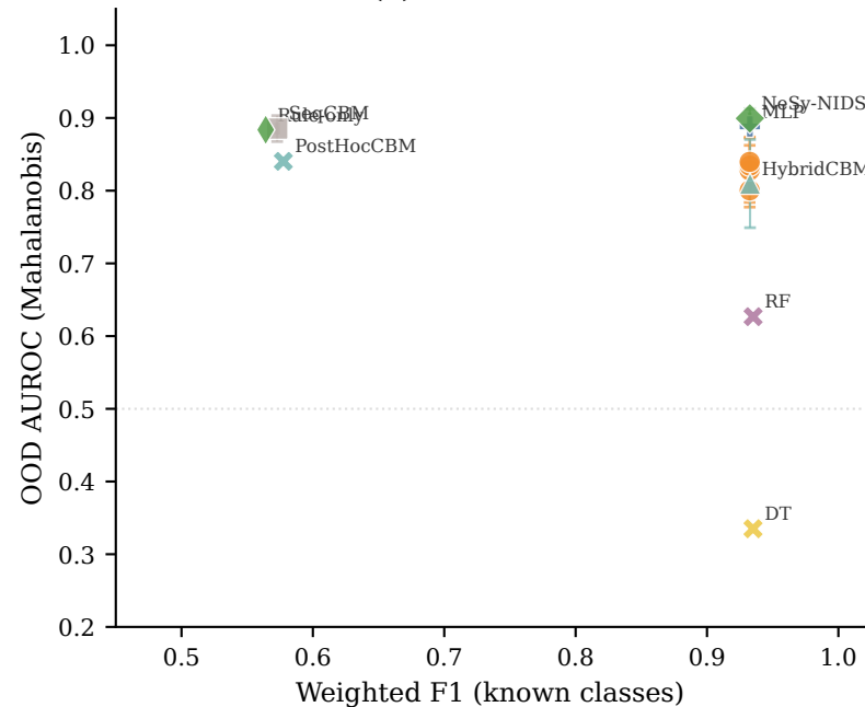
(a) CTU-IoT-23
