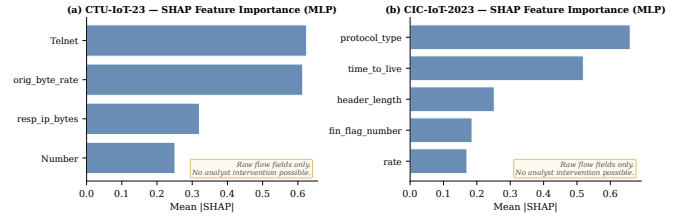
Fig. 6: SHAP mean |SHAP| feature importances for the MLP baseline on CTU-IoT-23 (left) and CIC-IoT-2023 (right). Top features are raw flow-level statistics ( Telnet , orig_byte_rate , protocol_type , time_to_live ) for which no analyst intervention is possible at inference time, in contrast to the directly overridable concept and rule activations of CBM and NeSy-NIDS.
