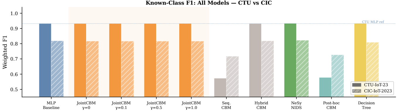
Fig. 2: Known-class weighted F1 for all models on CTU-IoT-23 (solid) and CIC-IoT-2023 (hatched). The shaded group covers the full \gamma \in \{0, 0.1, 0.5, 1.0\} ablation; all four variants sit at the same F1 as the MLP baseline, confirming that \gamma -regularisation affects only OOD detection (see Table II). SequentialCBM and Post-hoc CBM incur large F1 penalties on CTU from decoupled bottleneck training.
