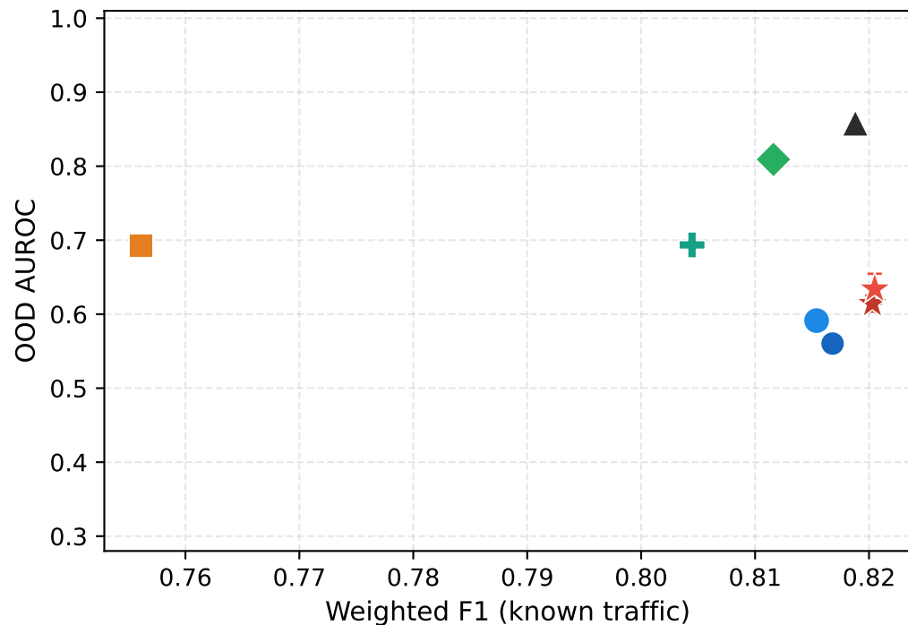
CIC-IoT-2023
