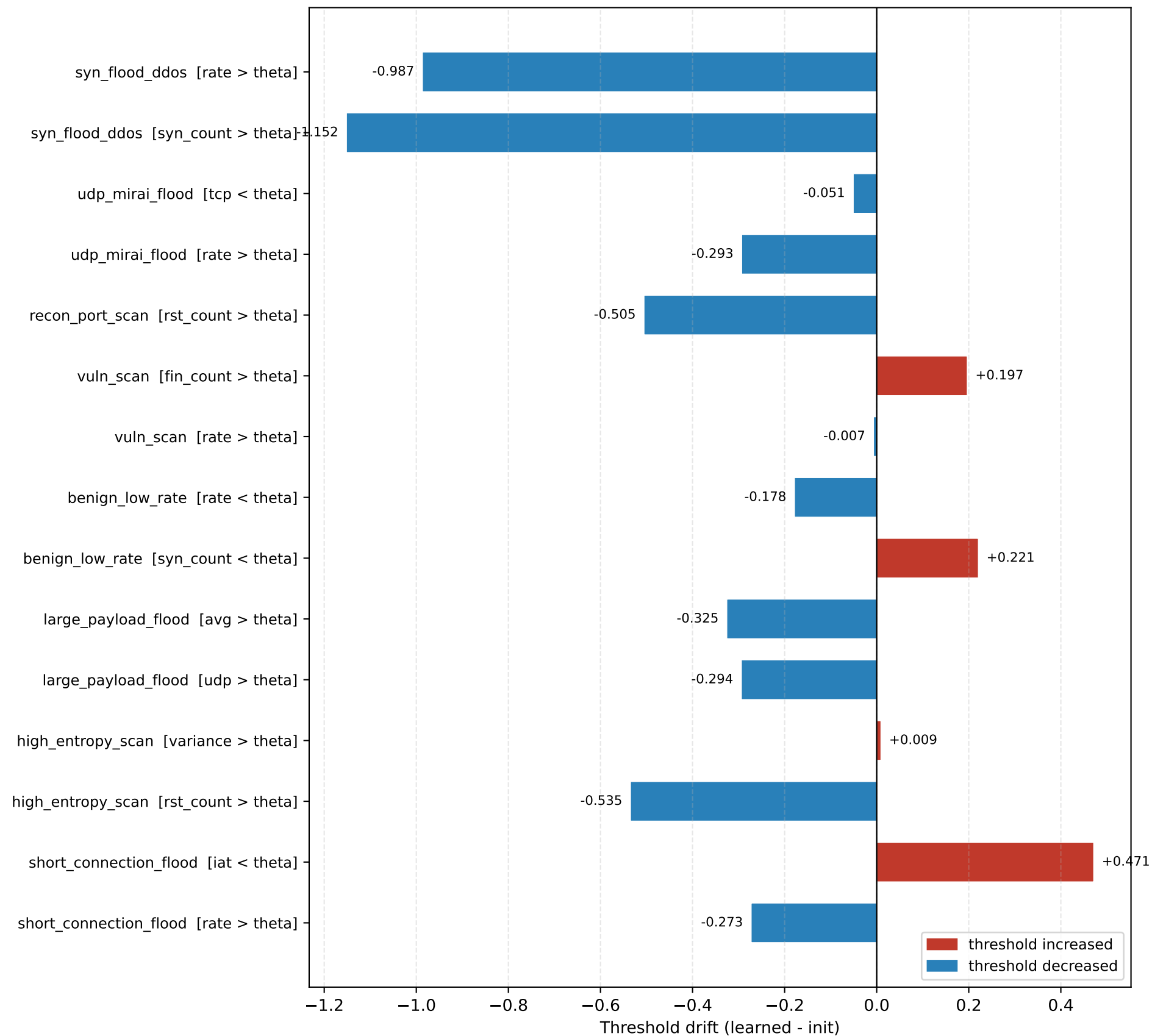
Learned Threshold Drift - CIC
