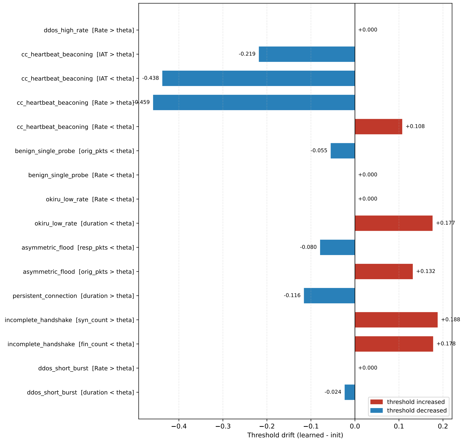
Learned Threshold Drift - CTU
