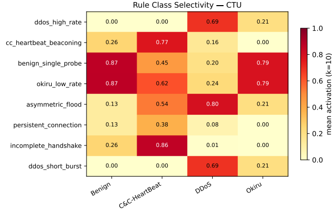
(a) CTU-IoT-23
