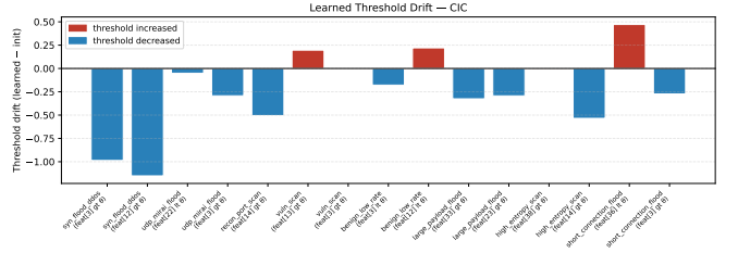
(b) CIC-IoT-2023
