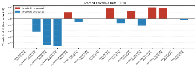
(a) CTU-IoT-23
