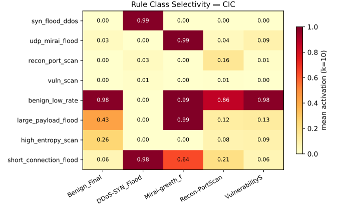
(b) CIC-IoT-2023
