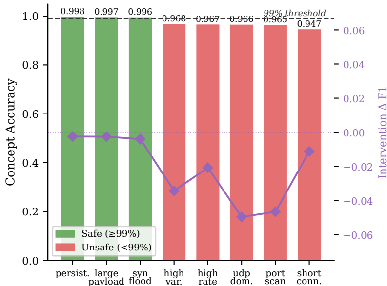
(b) CIC-IoT-2023 (JointCBM \gamma=0.5 )
