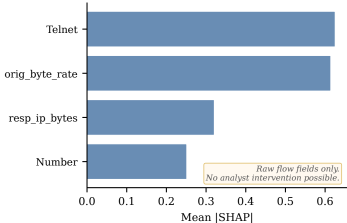
(a) CTU-IoT-23 — SHAP Feature Importance (MLP)
