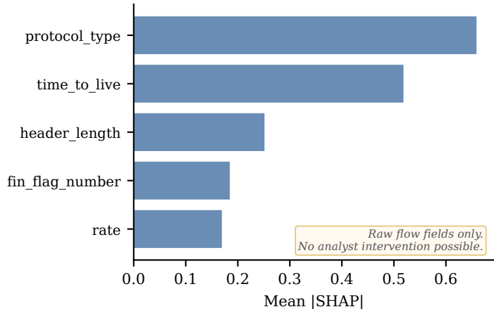
(b) CIC-IoT-2023 — SHAP Feature Importance (MLP)
