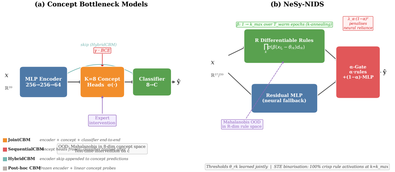
Fig. 1: System architectures. (A) Concept Bottleneck Model (CBM) : A 2-layer MLP concept encoder transforms raw features into K interpretable concept scores; a linear classifier maps concept scores to class logits. Predictions are fully auditable at the concept layer, and expert intervention can override individual concept values at test time. (B) NeSy-NIDS : Expert-defined threshold rules are differentially parameterised; k -annealing and the STE produce strictly binary rule activations at inference. A learnable \alpha -gate blends the rule head with a parallel neural fallback.
