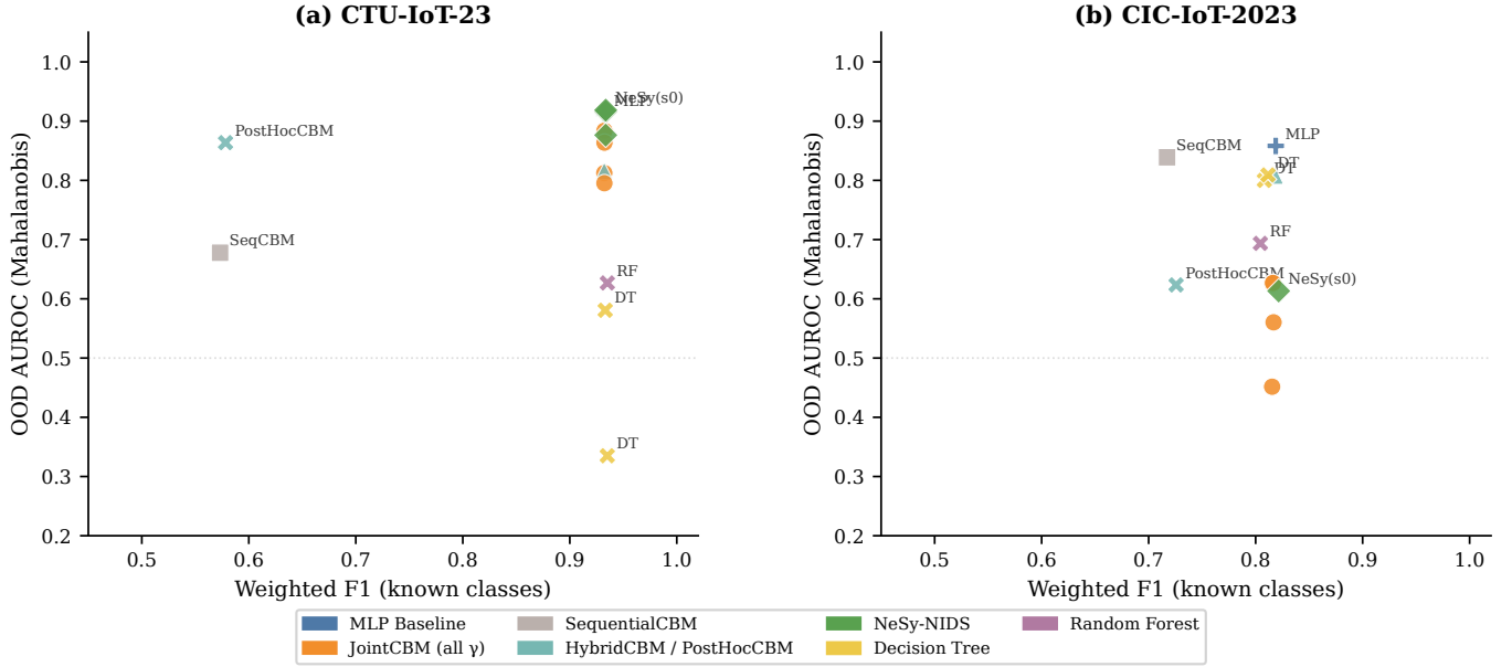
Fig. 3: OOD AUROC vs. known-class weighted F1 for all models on CTU-IoT-23 (left) and CIC-IoT-2023 (right). Error bars indicate \pm 1 std over 5 seeds where available.
