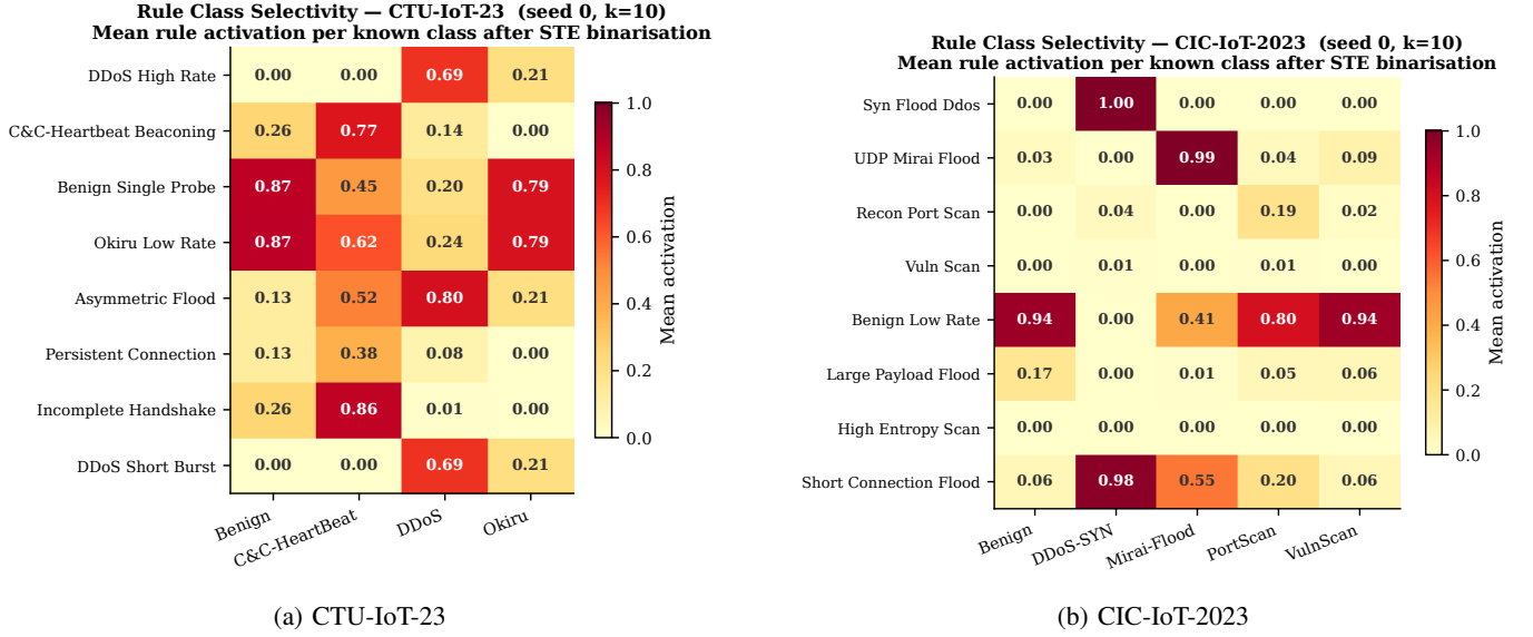
Fig. 4: Rule class selectivity heatmaps. Cell values are mean rule activation per class at k=10 (post-STE). Darker cells indicate more selective activation for that class.
