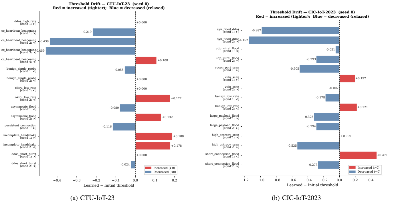
Fig. 5: Learned threshold drift (learned – initial) per rule condition. Red (positive) indicates the threshold increased; blue (negative) indicates it decreased.
