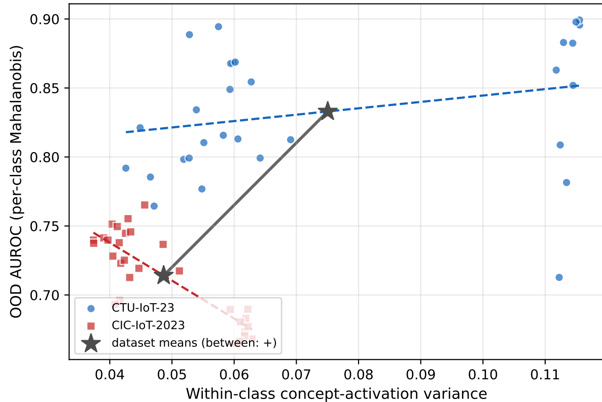
Within-class variance does not govern detectability
