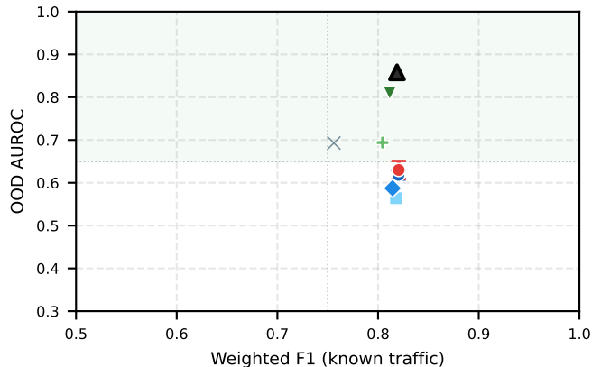
CIC-IoT-2023
