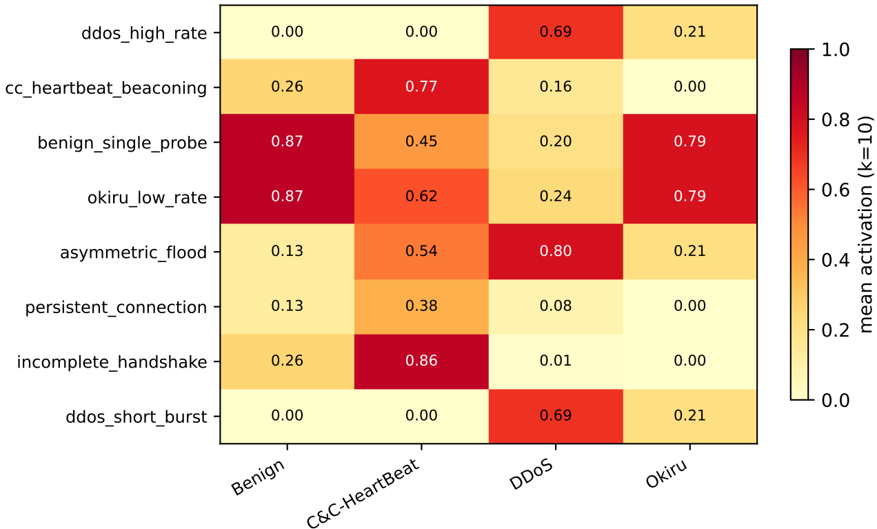
Rule Class Selectivity — CTU
