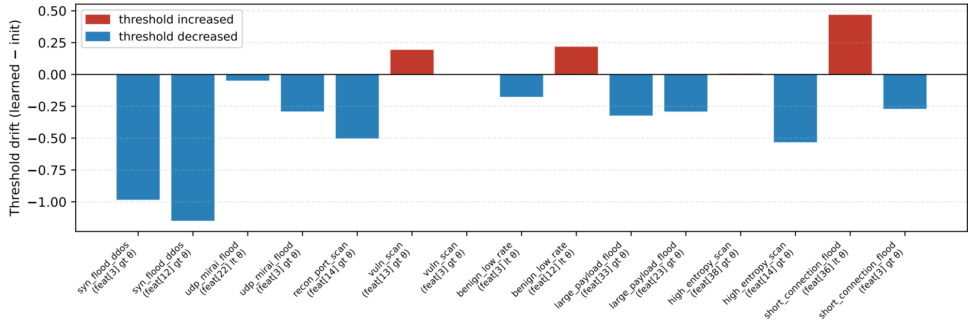
Learned Threshold Drift — CIC
