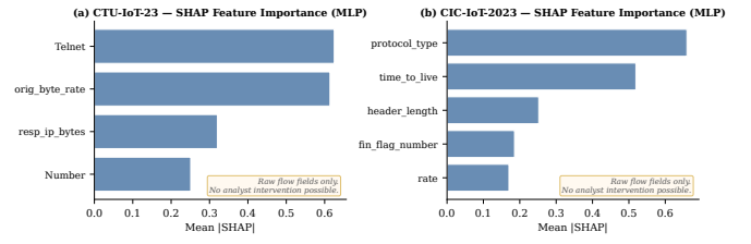
Fig. 6: SHAP mean |\text{SHAP}| feature importances for the MLP baseline on CTU-IoT-23 (left) and CIC-IoT-2023 (right). Top features are raw flow-level statistics ( Telnet , orig_byte_rate , protocol_type , time_to_live ) for which no analyst intervention is possible at inference time, in contrast to the directly overridable concept and rule activations of CBM and NeSy-NIDS.
