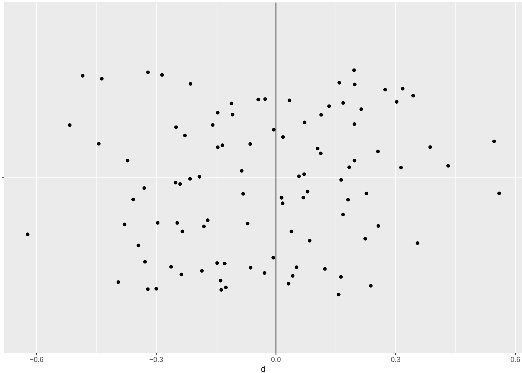
Distribution of effect sizes (two-sided t-test, N = 60 and a true effect of 0)
