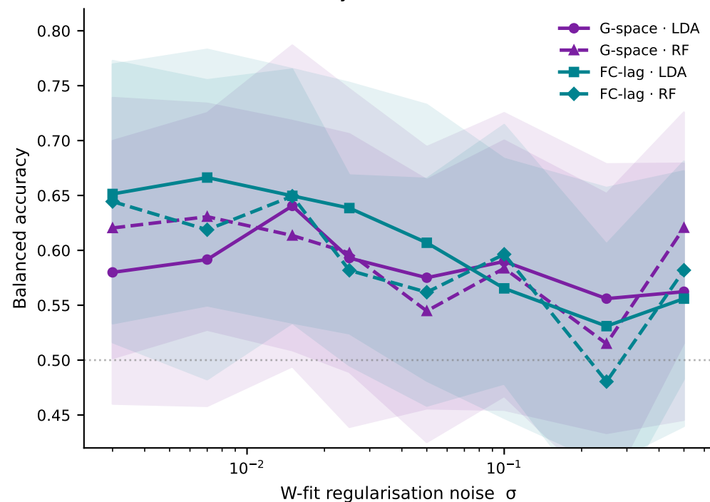
Accuracy vs. noise ( K = 15 )
