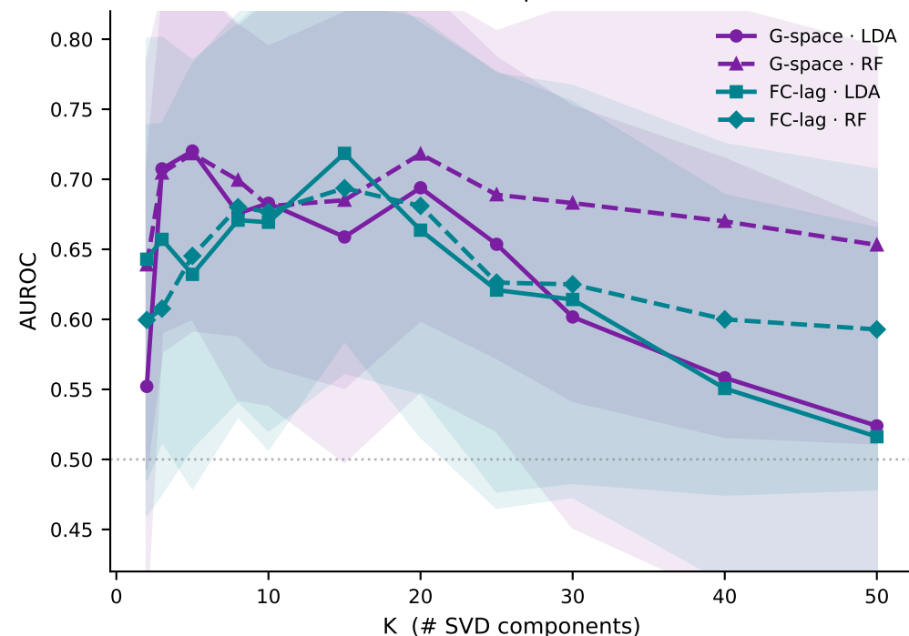
AUROC vs. # SVD components ( \sigma = 0.007 )
