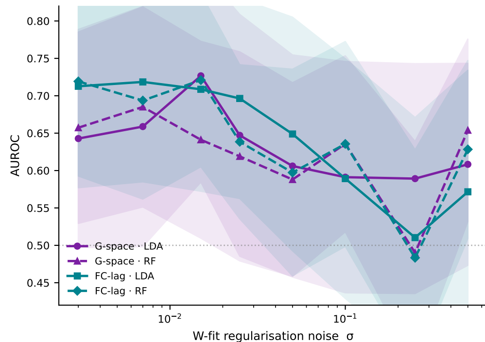
AUROC vs. noise ( K = 15 )
