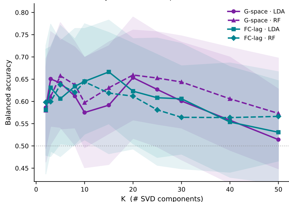
Accuracy vs. # SVD components ( \sigma = 0.007 )
