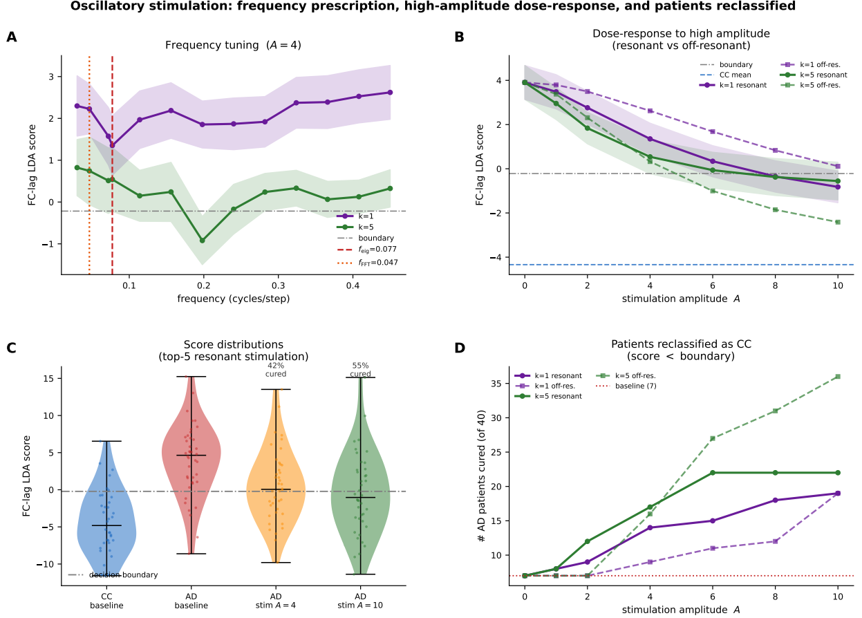
Figure S8. Frequency prescription and high-amplitude dose-response of focal oscillatory stimulation ( N = 40 AD). A sinusoidal drive A \sin(2\pi f t) is injected at the top- k most-affected ( \Delta W ) sites and the FC-lag score re-evaluated (lower = more control-like). (A) Frequency tuning at moderate amplitude ( A = 4 ): mean \pm SEM for the single top site ( k = 1 , purple) and the top-five sites ( k = 5 , green). For k = 1 the score is minimal precisely at the reservoir's dominant eigenmode frequency f_{\text{eig}} = 0.077 (red dashed), a sharp resonance; f_{\text{FFT}} (orange dotted) marks the spectral peak of the AD reservoir states. The k = 5 optimum broadens and shifts, as the FC-lag effect is a nonlinear functional of the dynamics, not the modal excitation amplitude. (B) Dose-response to high amplitude ( A = 10 ), resonant ( f_{\text{eig}} , solid) vs off-resonance (highest frequency, dashed) for k = 1 and k = 5 ; scores move toward the CC mean (blue dashed) as amplitude grows. (C) FC-lag score distributions: CC baseline, AD baseline, and AD after top-five resonant stimulation at A = 4 and A = 10 (decision boundary dot-dashed; fraction crossing it annotated). (D) Patients reclassified as CC vs amplitude, for top-1/top-5 \times resonant/off-resonant (baseline dotted): resonance is most efficient at low-to-moderate amplitude, whereas at supra-physiological amplitude even an off-resonance multi-site drive reclassifies most patients (36/40 at A = 10 ), an energy-driven (non-specific) saturation effect.
