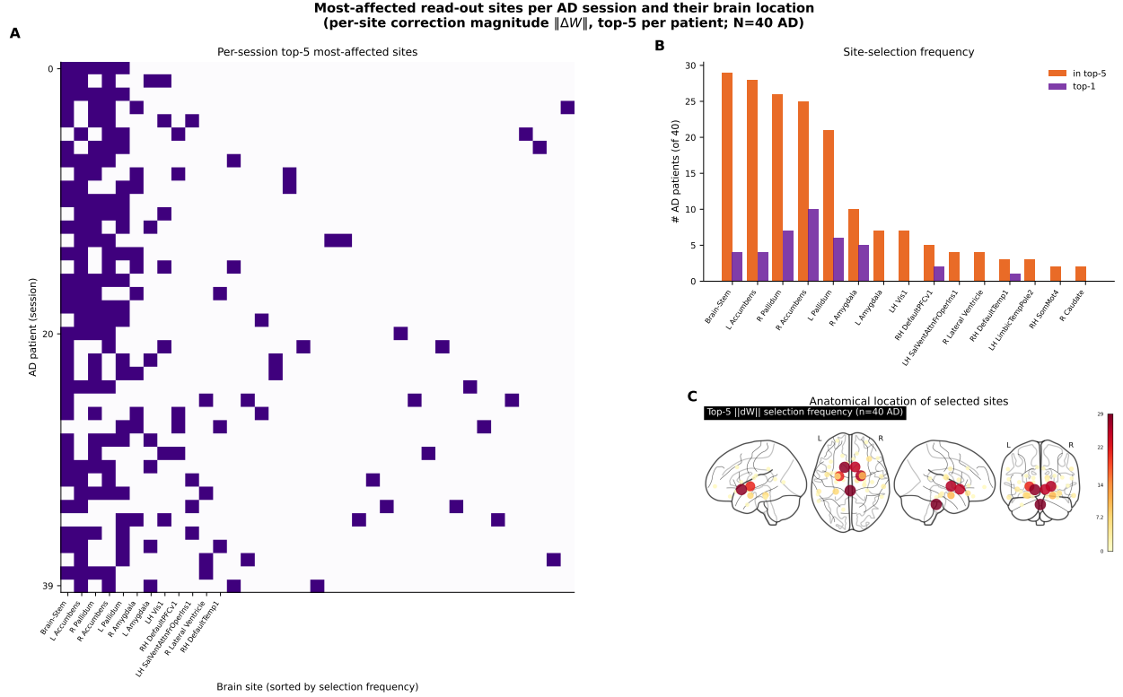
Figure 5. Most-affected read-out sites per AD session and their anatomical location. For each AD patient, brain sites are ranked by the per-site correction magnitude \|\Delta W\| (column norm of \Delta W = \bar{W}_{CC} - W_{AD} ). (A) Top-5 membership matrix: rows, the N = 40 AD sessions; columns, the brain sites ever selected, ordered by selection frequency; a filled cell marks a site among that patient’s top-five. (B) Selection frequency: number of AD patients with each site among the top-five (orange) or as the single most-affected site (top-1, purple). The leading sites are subcortical and limbic, bilateral pallidum and nucleus accumbens, the brainstem and the amygdala. (C) Glass-brain markers at the selected parcels (MNI centroids), coloured and sized by top-five selection frequency, showing their deep subcortical/limbic location.
