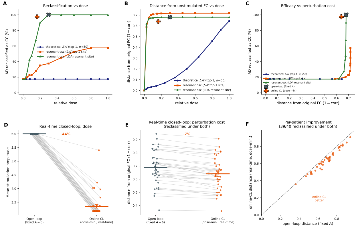
Fig. 5 | Single-site stimulation and closed-loop control ( N = 40 AD; distance = 1 - corr between the stimulated and unstimulated closed-loop free-run FC). Top row, single-site dose-response comparing a theoretical read-out correction ( \Delta W interpolation of the top-1 most-affected column toward the CC mean, \alpha \in [0, 50] ), a resonant drive A \sin(2\pi f_{\text{eig}} t) at that same \Delta W site, and a resonant drive at each patient's LDA-resonant (discriminant-aligned) site ( A \in [0, 20] ). (A) Reclassification vs normalised dose: the single-column \Delta W correction is inert (flat at the 18% baseline even at \alpha = 50 ); the resonant drive at the \Delta W site saturates near \sim 57\% ; the resonant drive at the LDA-resonant site reverts all patients (100%). (B) Distance from the original FC: the \Delta W correction distorts only gradually, whereas both resonant drives jump to \sim 0.7 at the smallest effective amplitude and saturate (the oscillation dominates the network-wide mode). (C) Efficacy vs perturbation cost: only the LDA-resonant drive converts perturbation into full reclassification. The closed-loop operating points (patient means; grey \times open-loop, orange + online closed-loop) are overlaid on A–C: the online closed-loop point sits at a substantially smaller dose than the open-loop point, for a comparable, though not quite complete (97.5% vs 100%), reclassification rate and a modestly smaller distance. Bottom row, real-time closed-loop control at the LDA-resonant target (the same curing site as the green curve of A), comparing a fixed open-loop drive ( A = 6 ) to an online closed-loop controller that titrates amplitude every few steps from a sliding-window estimate of the FC-lag biomarker computed only from the model's own past output, no oracle access to the future trajectory (Methods). (D) Per-patient stimulation amplitude (dose): online control lowers the mean dose from 6.0 to 3.3 ( \sim 44\% lower) while nearly matching efficacy (39/40, 97.5%, vs 40/40 open-loop). (E) Distance from baseline among patients reclassified under both protocols ( n = 39 ): online control lowers the mean distance by \sim 7\% ( 0.69 \rightarrow 0.64 ). (F) Per-patient: most subjects lie below the diagonal, i.e. real-time control reaches nearly the same reversal at a smaller perturbation cost, the in-silico analogue of adaptive (closed-loop) neuromodulation, using only information available causally, online.
