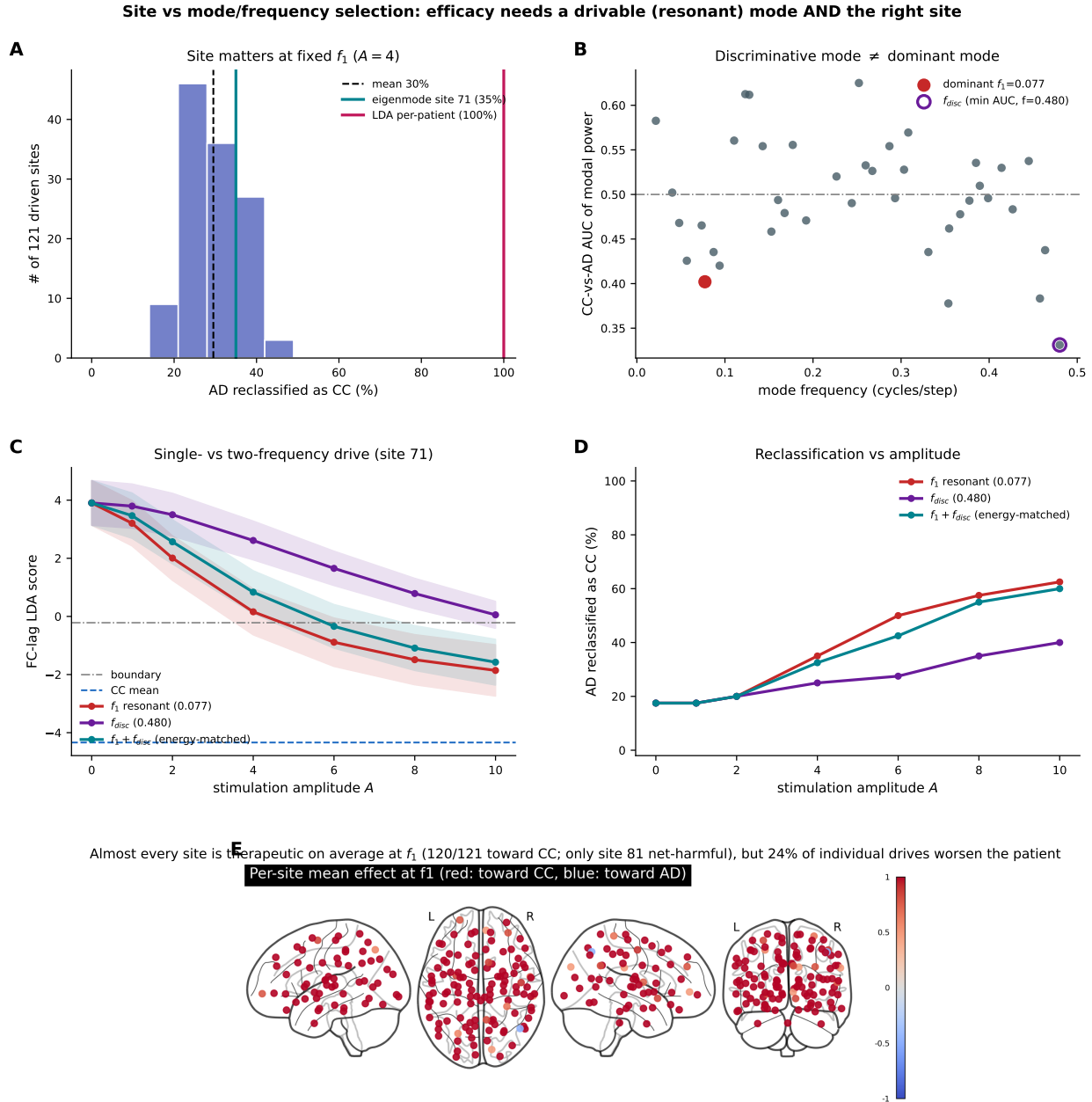
Figure S7. Why site and resonance both matter: a drivable mode is not the same as a disease-discriminative one
