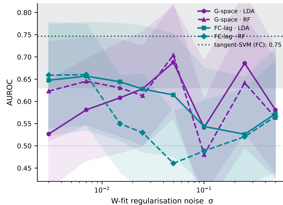
AUROC vs. noise ( K = 25 )
