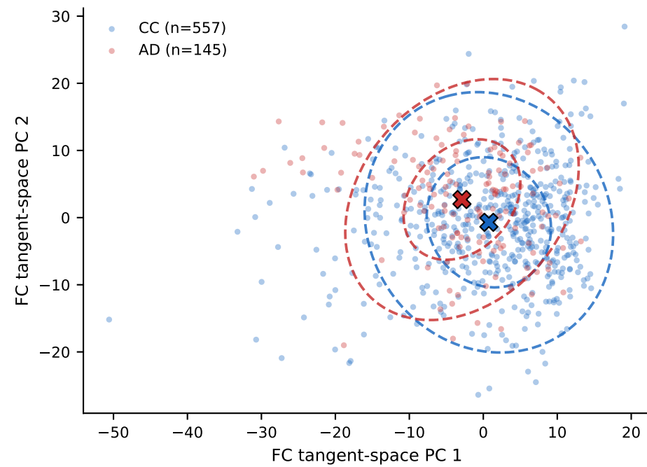
CC vs AD point clouds (2-D PCA of FC features)
