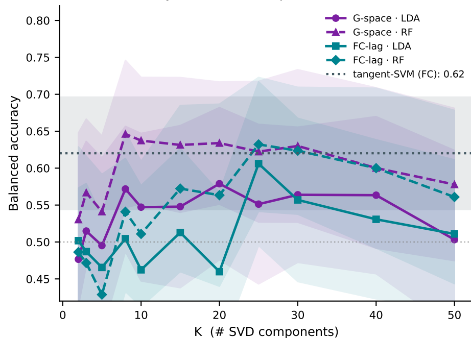
Accuracy vs. # SVD components ( \sigma = 0.007 )
