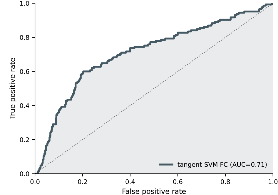
Tangent-space FC benchmark --- ROC (nested 5×5 patient-level CV)
