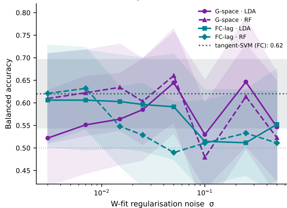
Accuracy vs. noise ( K = 25 )
