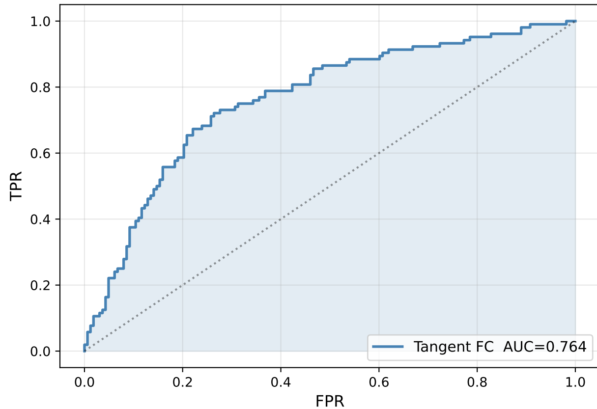
Tangent-space FC — CN vs AD (nested 5×5 CV, patient-level groups)
