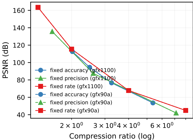
ZFP quality vs. ratio, TTI 4GB
