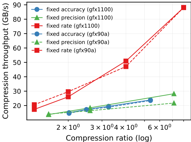
ZFP throughput vs. \ ratio, TTI 4GB
