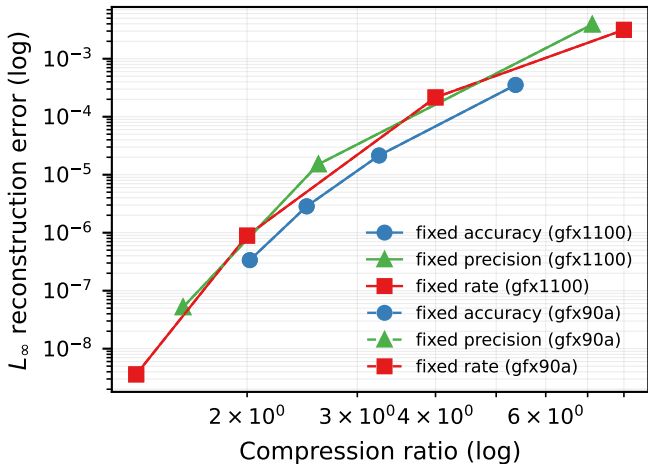
ZFP error vs. \ ratio, TTI 4GB
