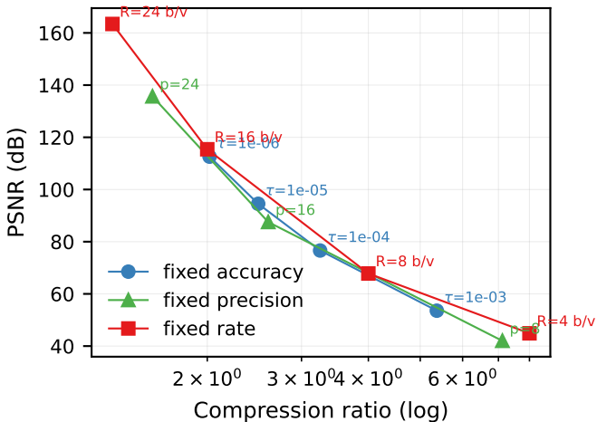
ZFP quality vs. ratio, TTI 4 GiB, gfx1100
