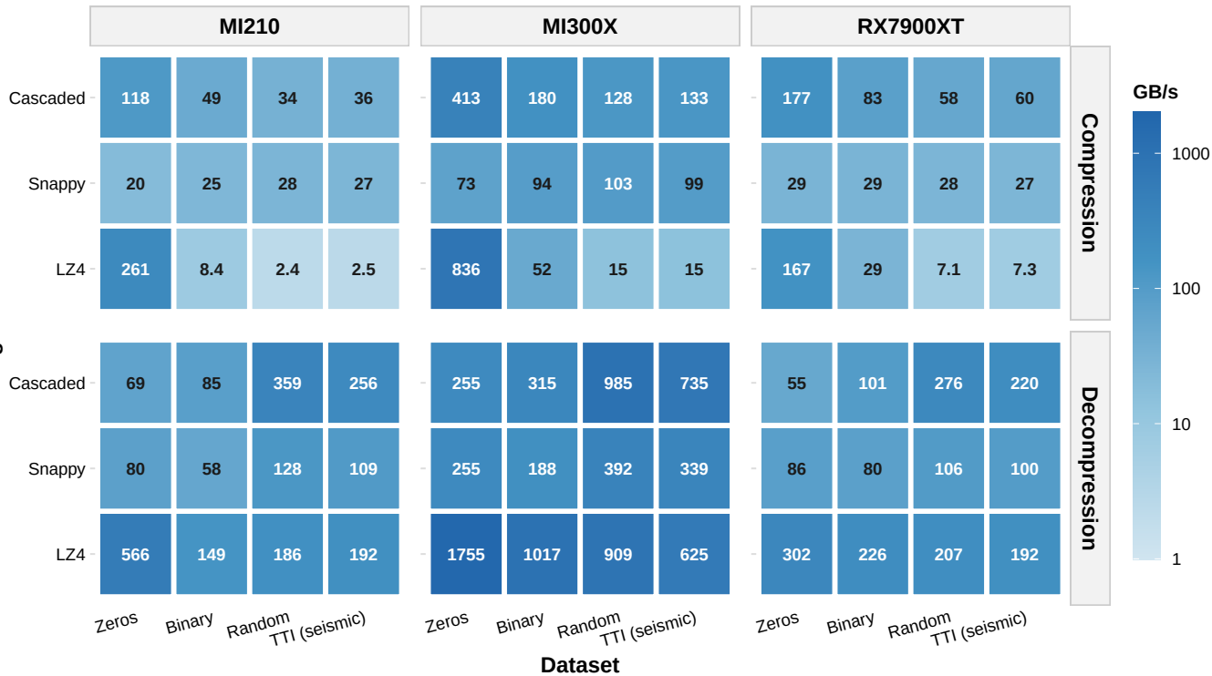
Algorithm
