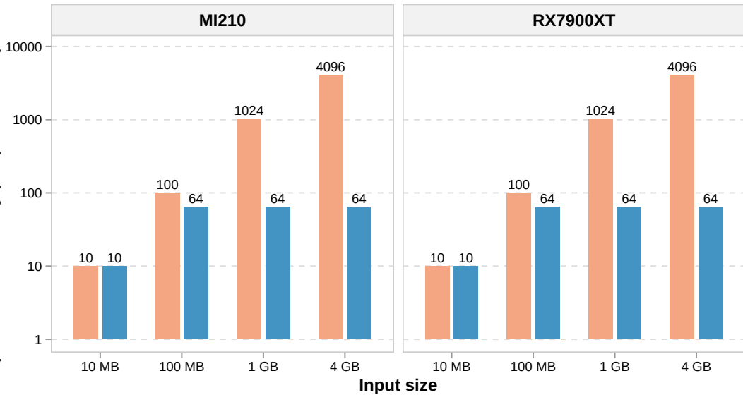
Peak pinned host memory (MiB) - LZ4/TTI (seismic)
