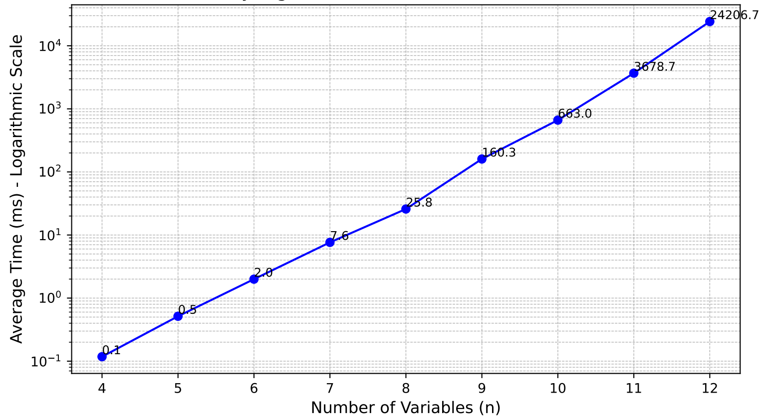
Quine-McCluskey Algorithm Performance: Runtime vs. Variables (n)
