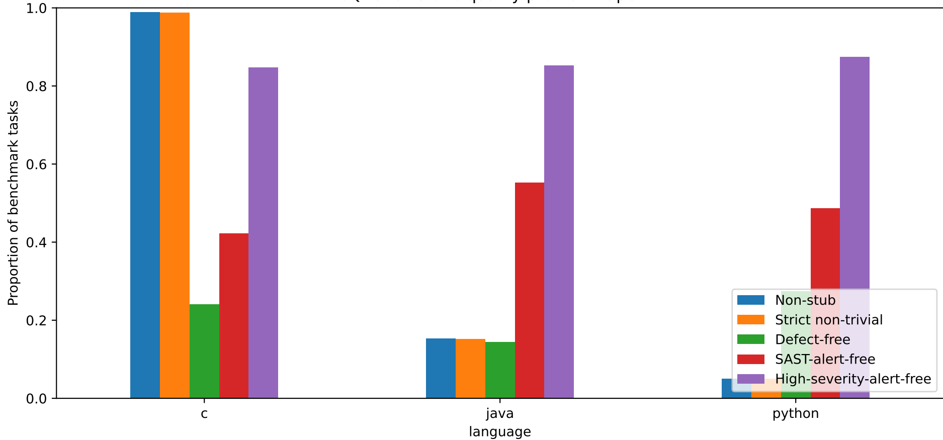
CQBench static quality profile — OpenAI
