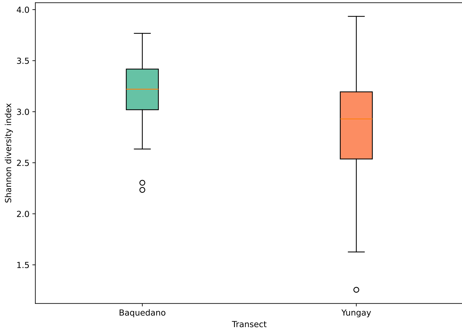
Shannon diversity by transect
