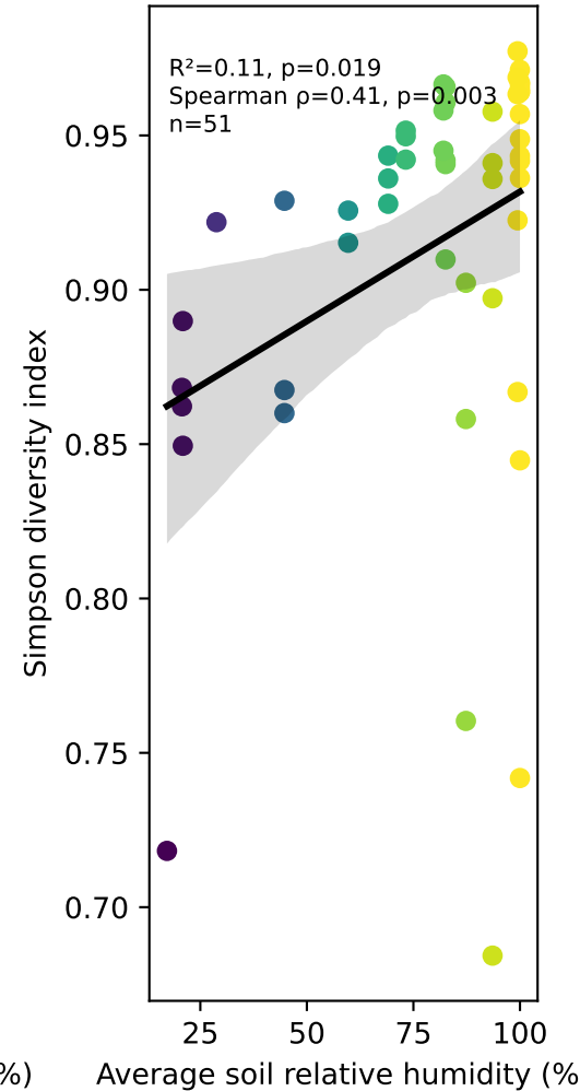
Simpson diversity index
