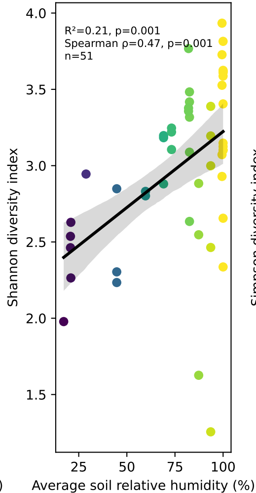
Shannon diversity index
