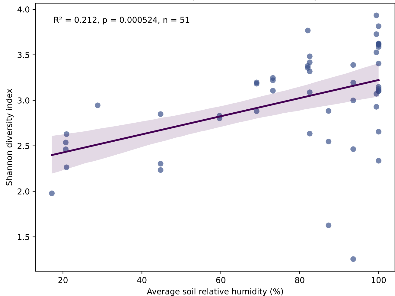
Shannon diversity vs. soil relative humidity
