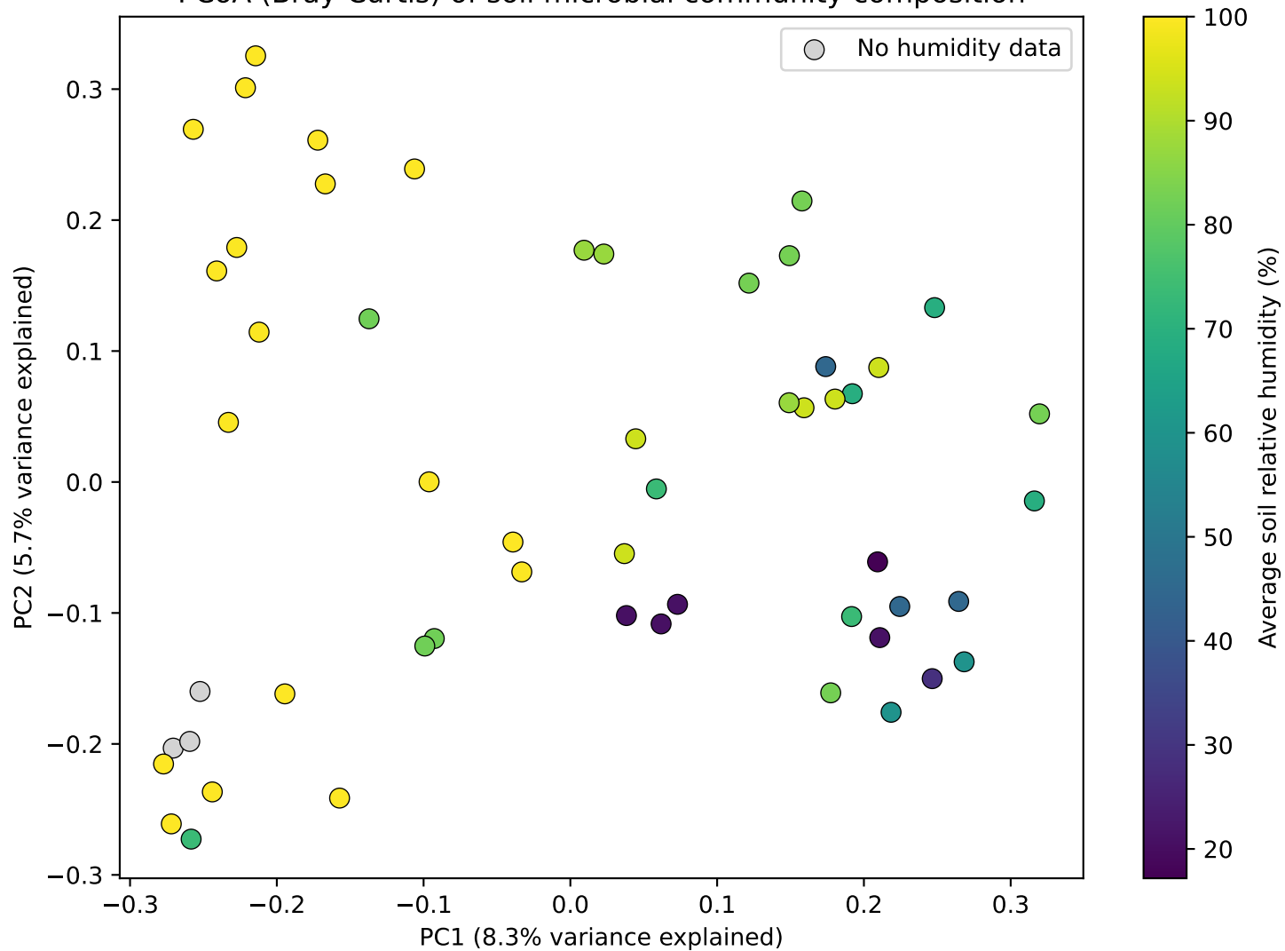
PCoA (Bray-Curtis) of soil microbial community composition
