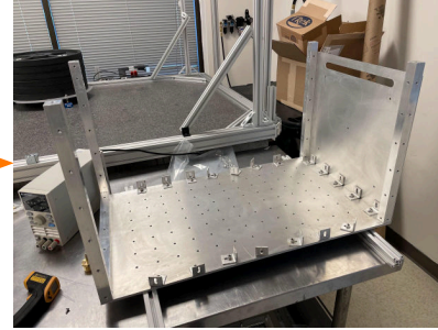
Mechanical Integration
