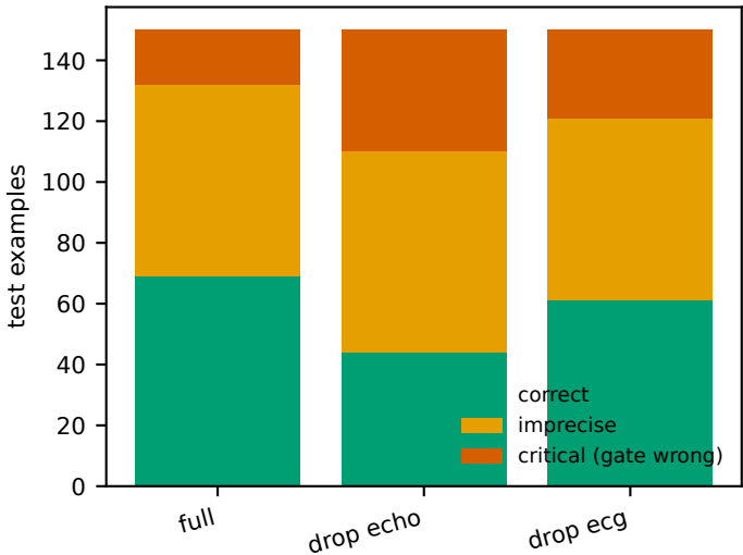
Failure taxonomy by condition
