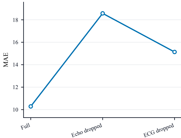
(a) LVEF regression
