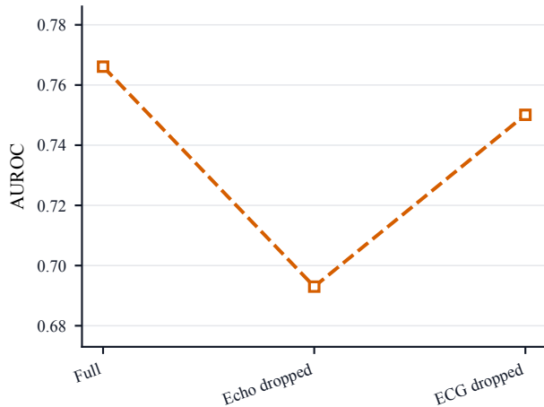
(b) EF \leq 40\% classification
