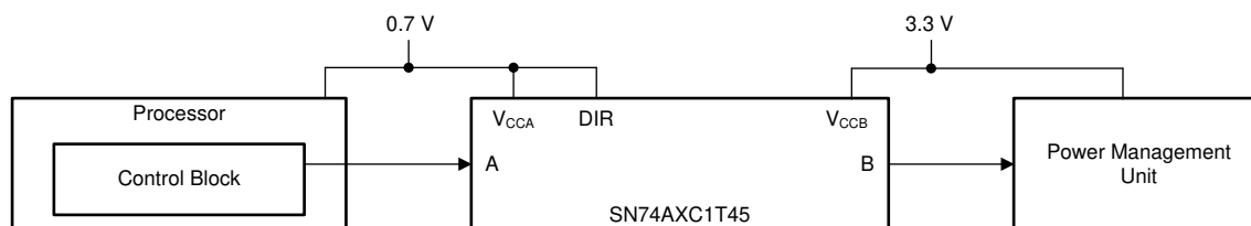
Simplified Schematic
