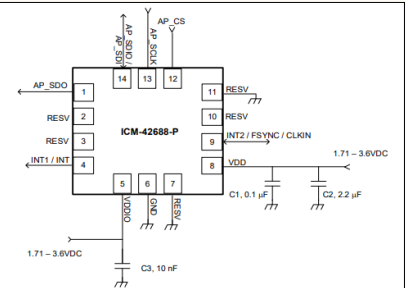
Figure 6. ICM-42688-P Application Schematic (SPI Interface to Host)
