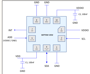
Figure 10. ICP-20100 Application Schematic (I2C / PC Interface to Host)
