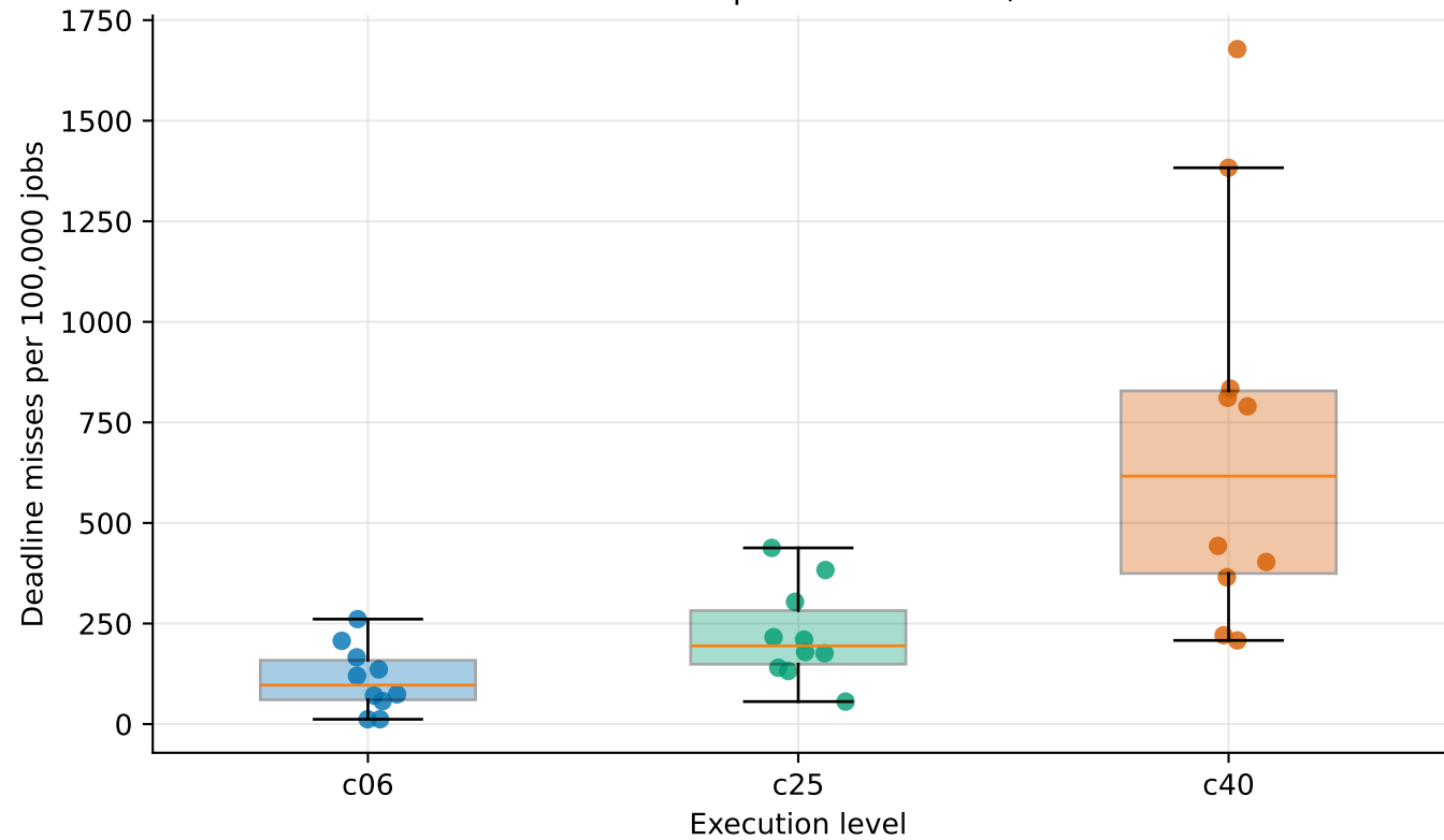
Deadline-miss amplification under I/O stress
