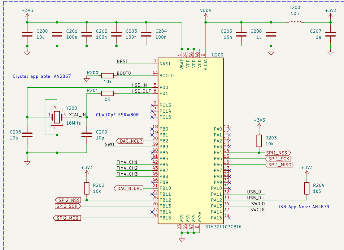
MCU (STM32F1)
