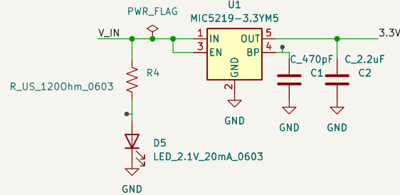
LDO REGULATOR (ULTRA LOW NOISE IMPLEMENTATION)
