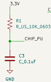
RC DELAY CIRCUIT (DELAYED POWER ON)
