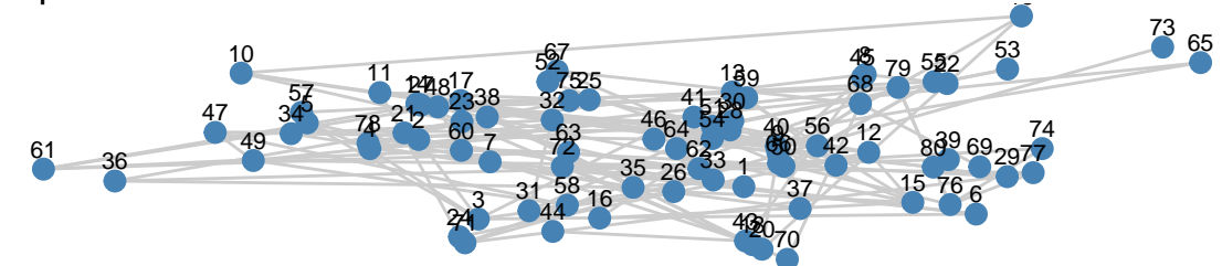
* Hybrid
