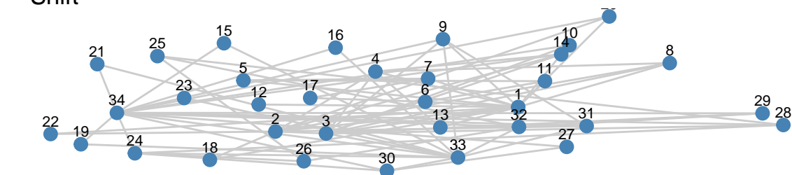
* Dp
