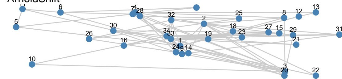
* ArnoldShift
