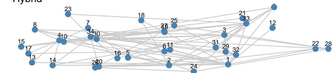
* Hybrid
