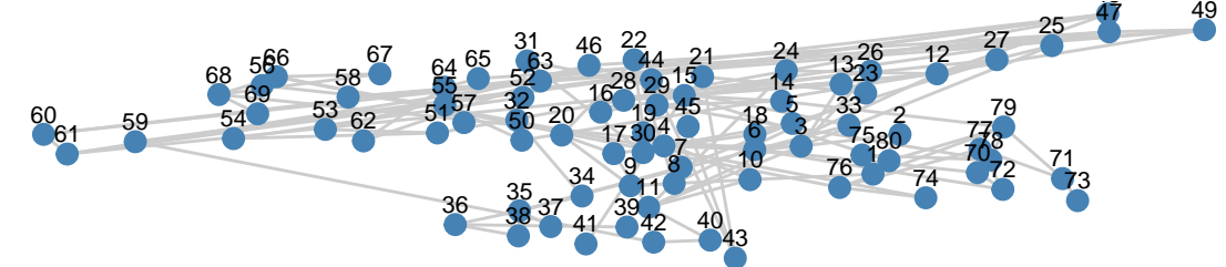
* Dp
