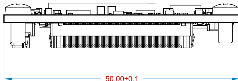
View from Front side (Scale 2:1)
