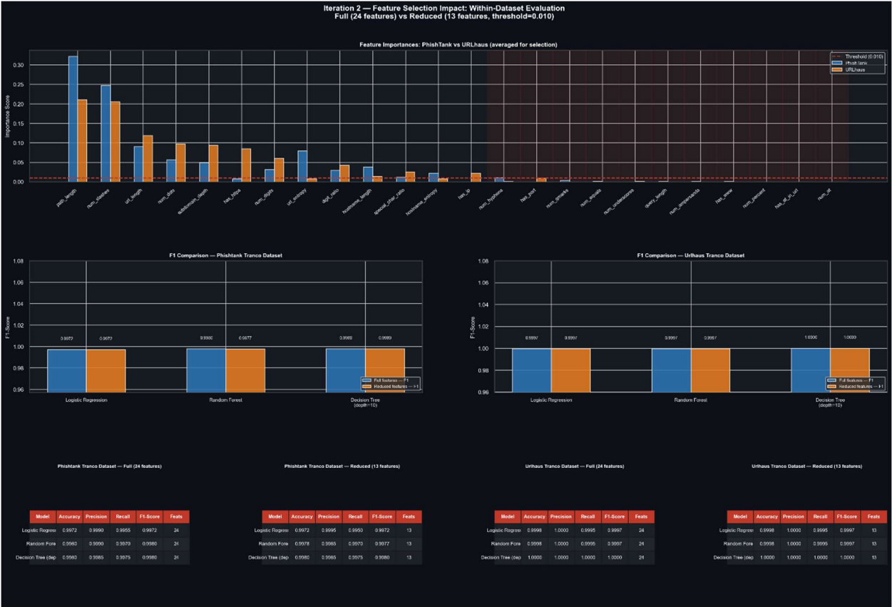
Figure 6 Feature Selection Impact Dashboard: Within-Dataset Evaluation (Iteration 2) Side-by-side comparison of full 24-feature and reduced 13-feature performance across all three classifiers on both datasets, including feature importance bar charts with the 0.01 threshold line and \Delta F1 annotations. Generated by feature_selection_eval.py and saved as dashboard_feature_selection_within.png in the outputs/ directory.
