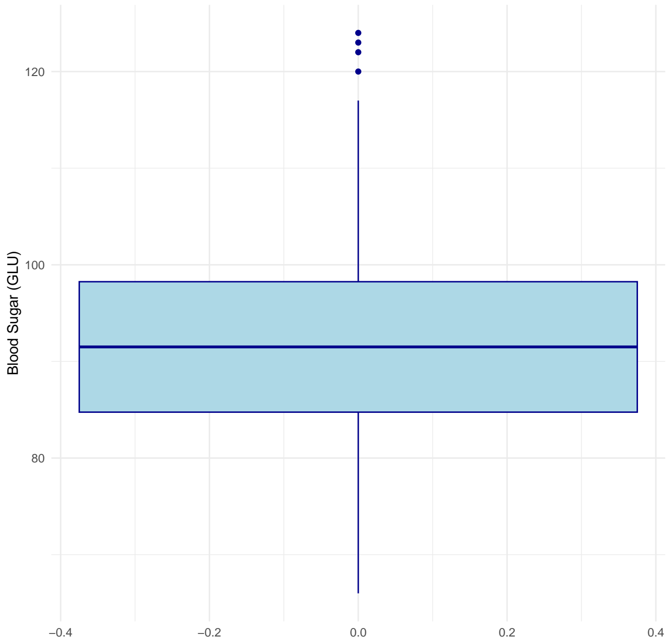
Box Plot of Blood Sugar (GLU)
